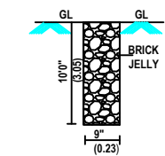
PERCULATION PIT
