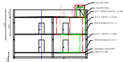
CUT SECTION ON AA
