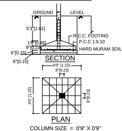
FOUNDATION DETAILS
