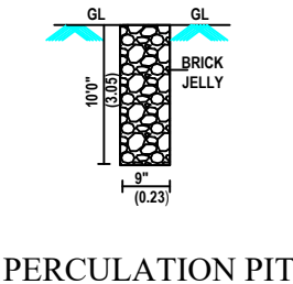
PERCULATION PIT
