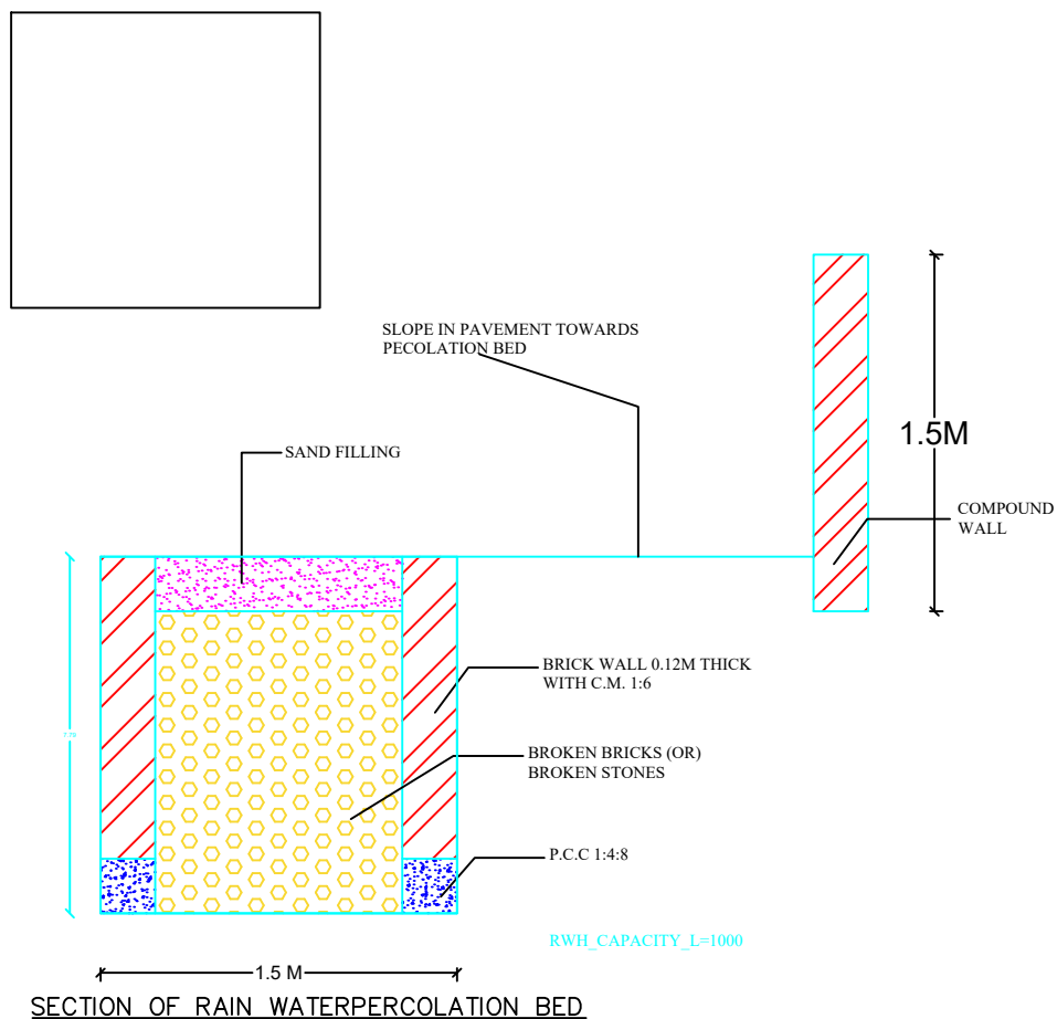
SECTION OF RAIN WATERPERCOLATION BED
