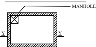
UG - SUMP DETAIL PLAN
