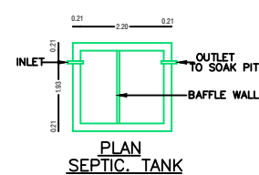
PLAN SEPTIC. TANK
