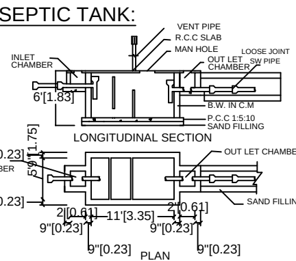
SEPTIC TANK:
