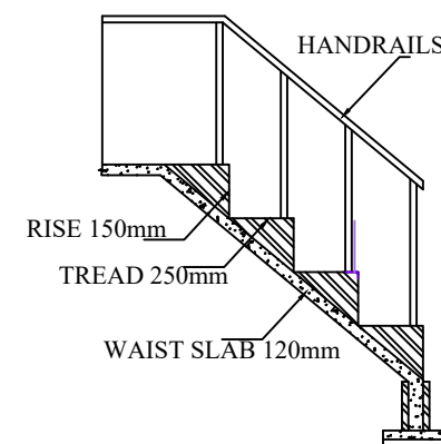
STAIRCASE DETAILS
