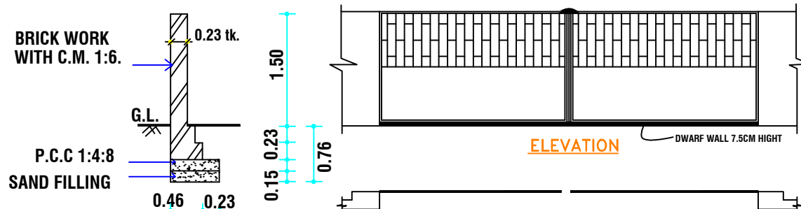
SECTION OF COMPOUND WALL
