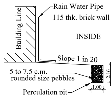
RAIN WATER HARVESTING PERCOLATION PIT
