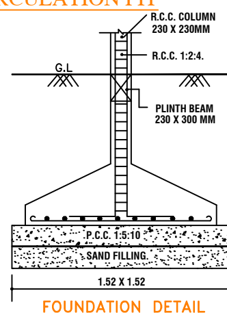
FOUNDATION DETAIL
