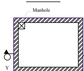
Sump Detail - Plan
