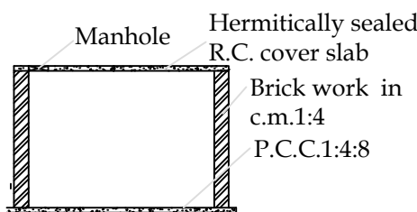
Section On 'Y-Y'
