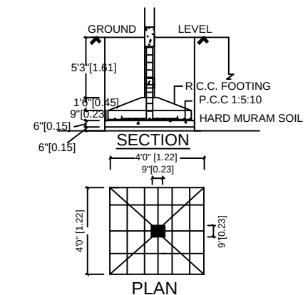
PLAN IN SIZE = 0'9" X 0'9"
