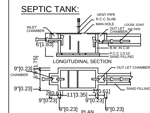
SEPTIC TANK:
