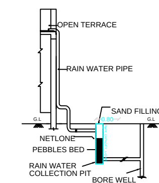
RAIN WATER HARVESTING SYSTEM
