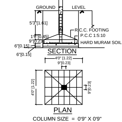
FOUNDATION DETAILS
