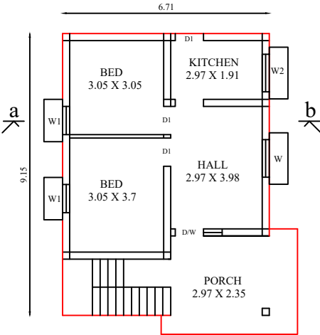
PROPOSED PLAN
