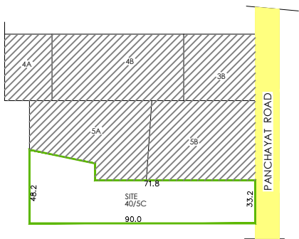
KEY PLAN SCALE:1"=132'0"
