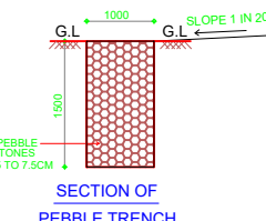
SECTION OF PEBBLE TRENCH SCALE : 1 : 100
