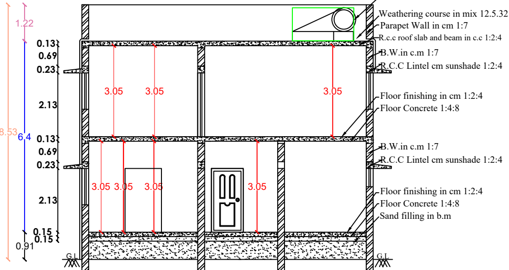
SECTION - "AB,CD"
