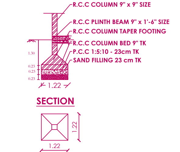
COMPOUND WALL DETAILS
