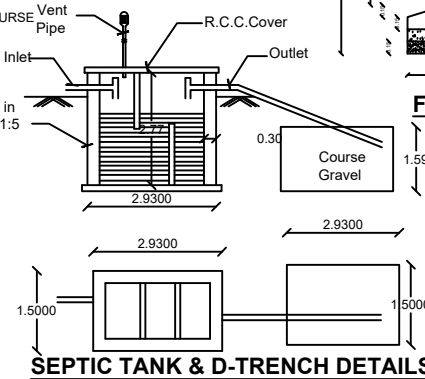
SEPTIC TANK & D-TRENCH DETAILS
