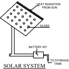
SOLAR SYSTEM
