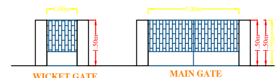
WICKET GATE
