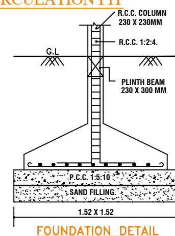
FOUNDATION DETAIL
