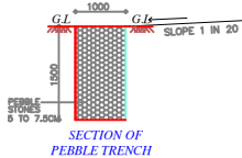
SECTION OF PEBBLE TRENCH
