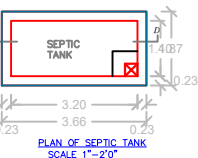
PLAN OF SEPTIC TANK SCALE 1"=20'
