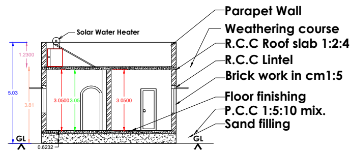
SECTION ON ABCD
