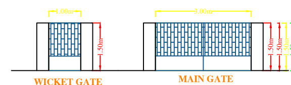
WICKET GATE
