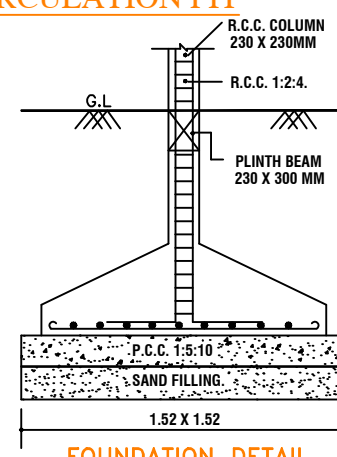
FOUNDATION DETAIL
