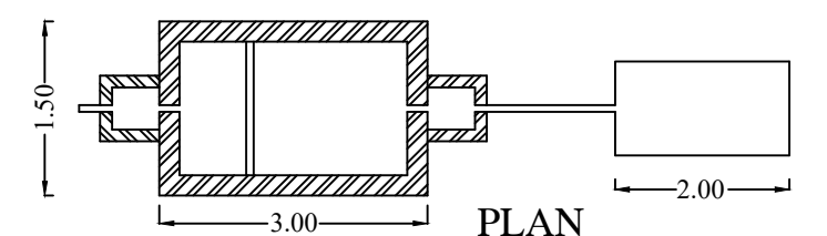
SEPTIC TANK DISPERSION TRENCH
