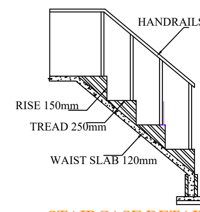
STAIRCASE DETAILS
