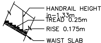
STAIRCASE DETAILS
