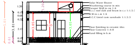
SECTION - "AB "
