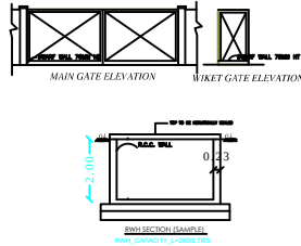
MAIN SECTION (SAMPLE) HIGH CAPACITY 3=200LITRES
