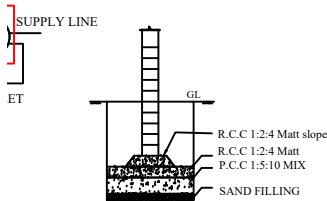
COLUMN DETAILS
