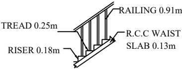
STAIRCASE DETAILS
