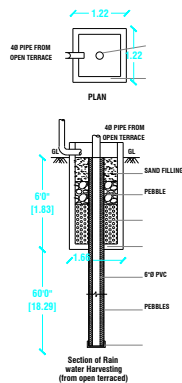
Section of Rain water Harvesting (from open terrace)
