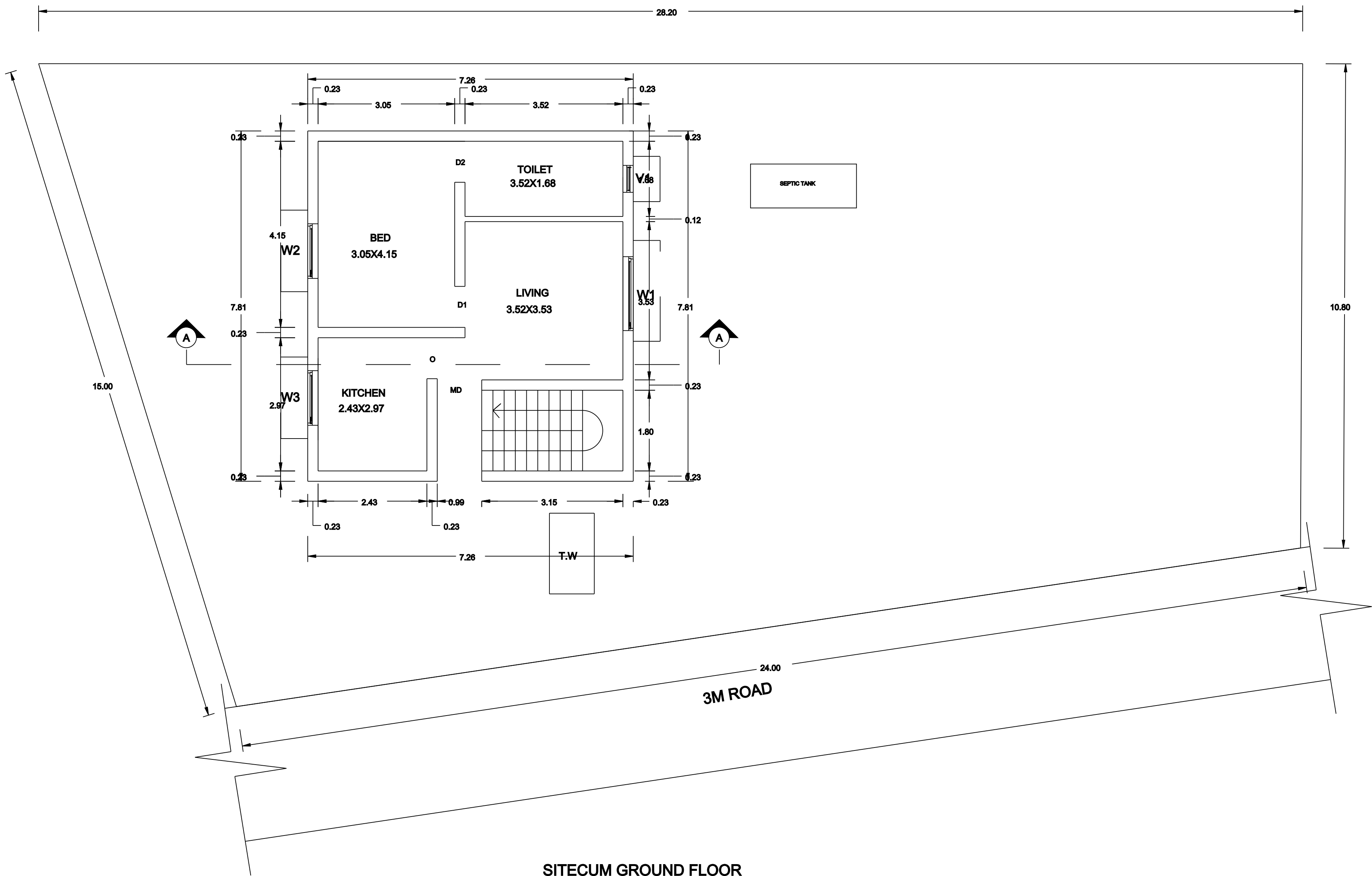
SITECUM GROUND FLOOR
