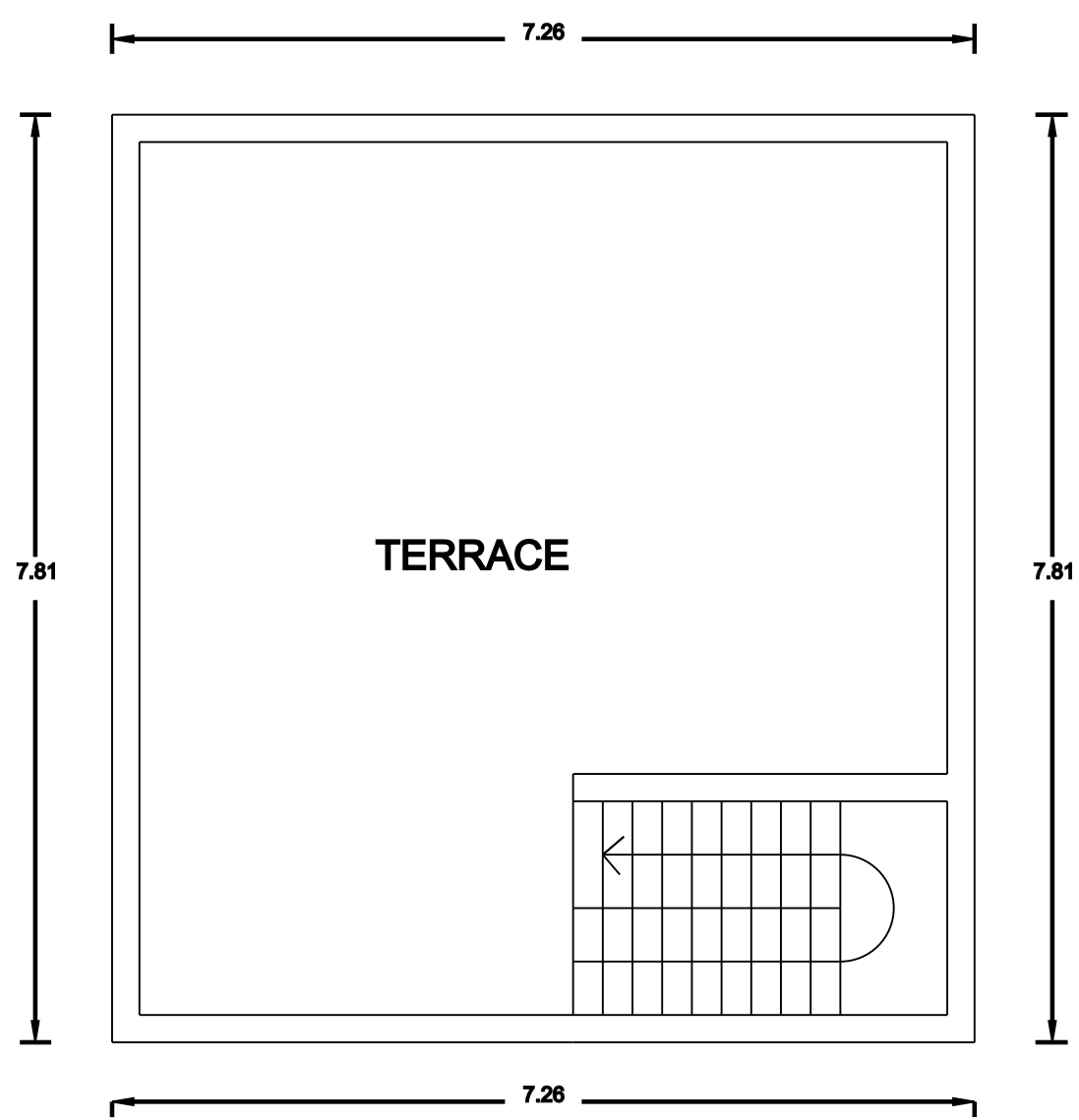
TERRACE FLOOR
