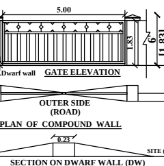
SECTION ON DWARF WALL (DW)
