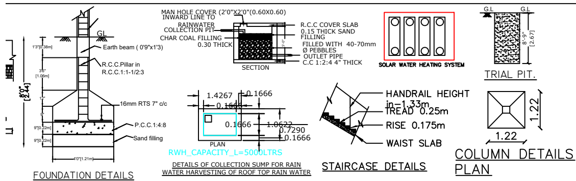
FOUNDATION DETAILS
