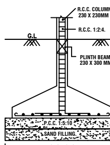
FOUNDATION DETAIL
