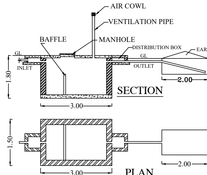
SEPTIC TANK DISPERSION TRENCH
