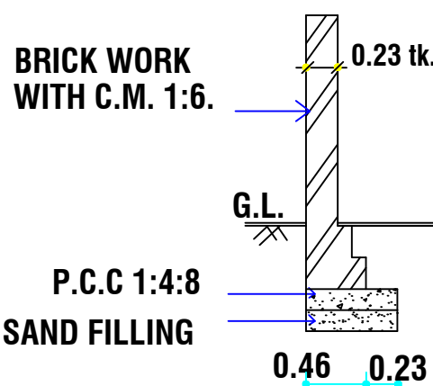
SECTION OF COMPOUND WALL
