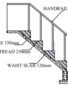
STAIRCASE DETAILS
