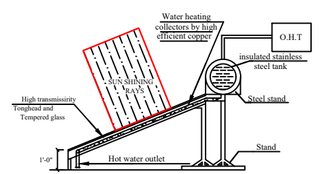
SECTION SOLAR WATER HEATER
