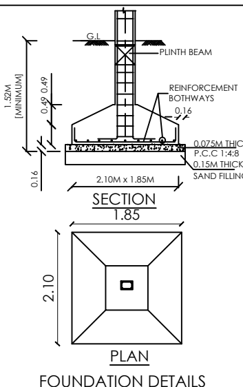
FOUNDATION DETAILS
