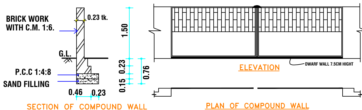
SECTION OF COMPOUND WALL
