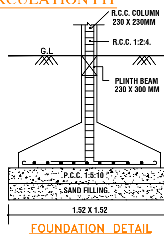
FOUNDATION DETAIL
