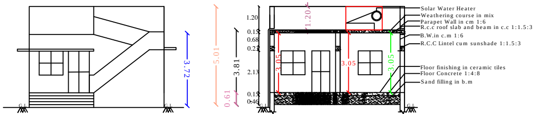
SECTION - "AB "
