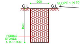
SECTION OF PEBBLE TRENCH SCALE : 1 = 100
