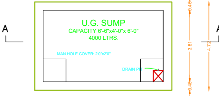
SUMP DETAIL
