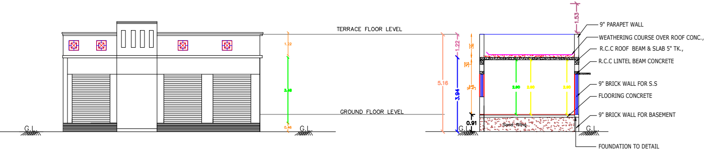
FRONT ELEVATION
