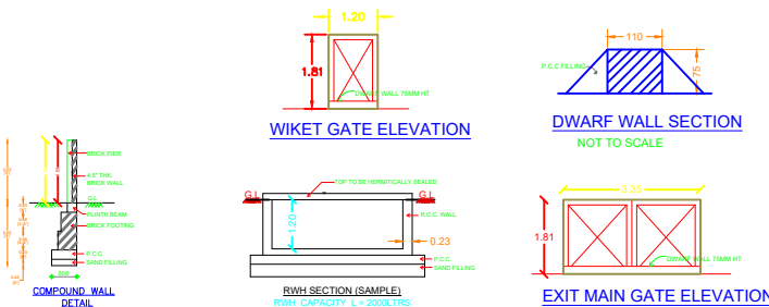
EXIT MAIN GATE ELEVATION
