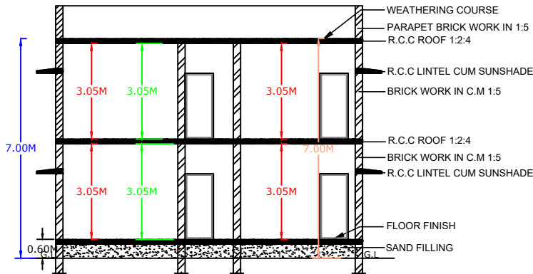
SECTION ON XX
