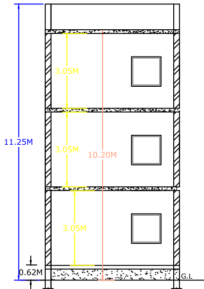
SECTION ON XX
