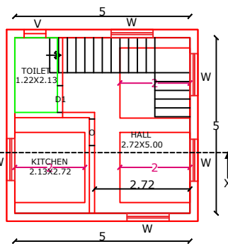
PRO.SECOND FLOOR PLAN
