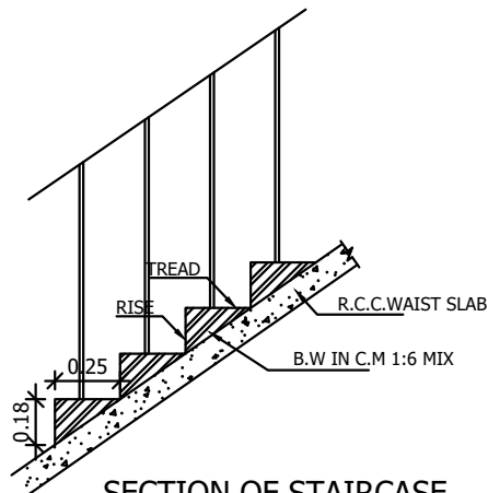
SECTION OF STAIRCASE
