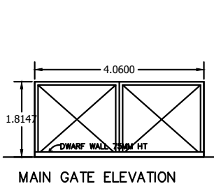
MAIN GATE ELEVATION
