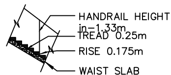
STAIRCASE DETAILS
