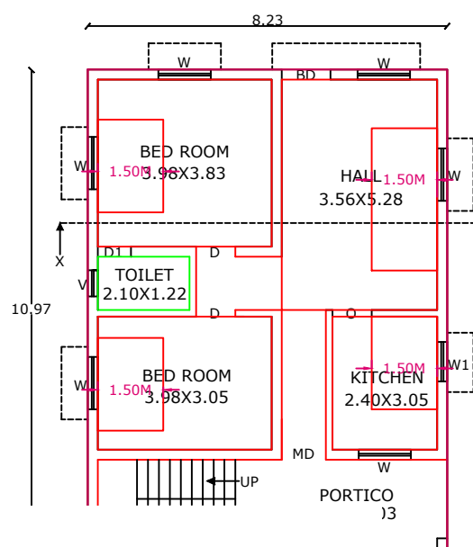
PLAN
