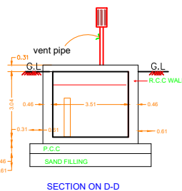
SECTION ON D-D
