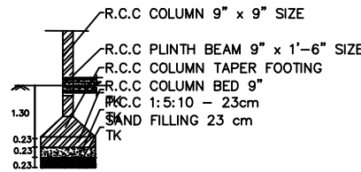
SECTION COLUMN DETAILS PLAN
