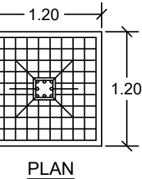
COLUMN FOOTING DETAILS
