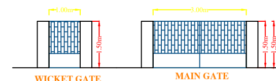
WICKET GATE
