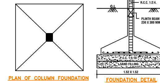
PLAN OF COLUMN FOUNDATION
