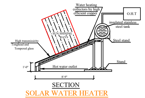
SECTION SOLAR WATER HEATER
