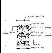
WASTE WATER RECYCL UNIT
