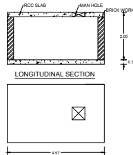
SUMP DETAILSUMP DETAIL
