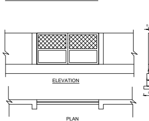
GATE & COMPOUND WALL DETAIL
