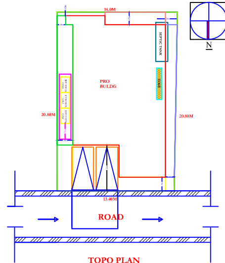
TOPO PLAN
