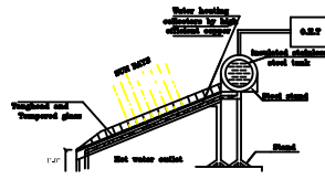
WATER HEATER
