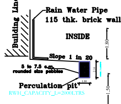
RAIN WATER HARVESTING PERCUSSION PIT
