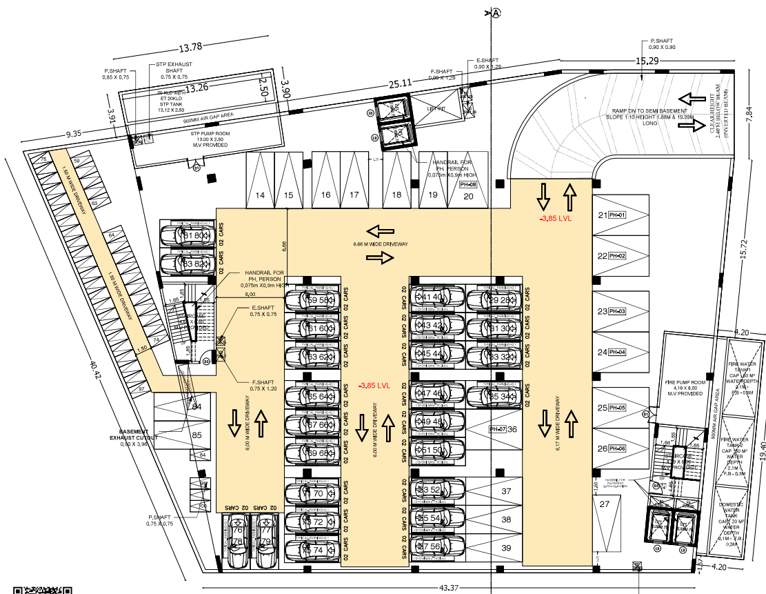
SEMI BASEMNET FLOOR PLAN
