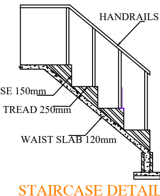
STAIRCASE DETAILS
