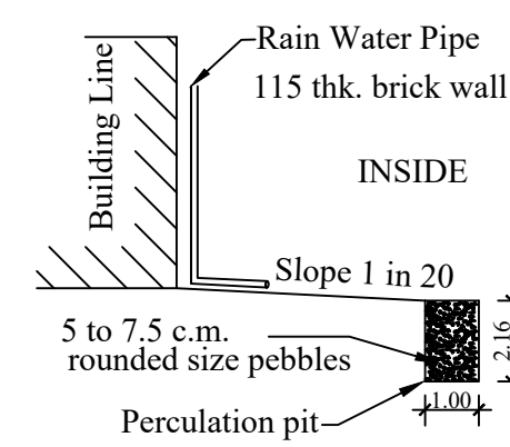
RAIN WATER HARVESTING PERCOLATION PIT
