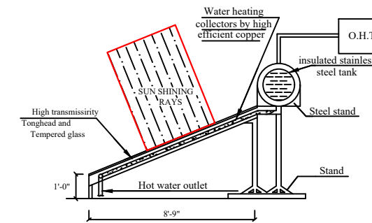
SECTION SOLAR WATER HEATER
