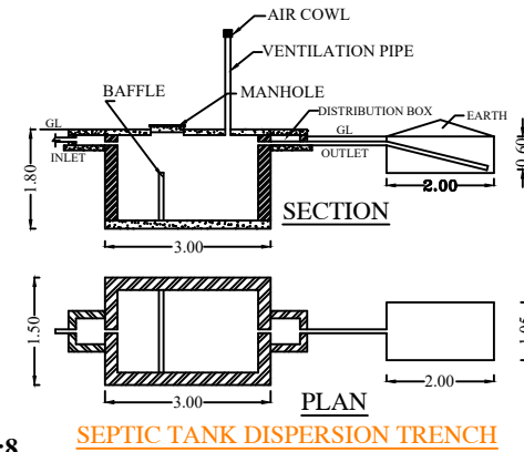
SEPTIC TANK DISPERSION TRENCH
