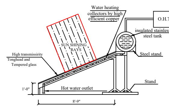
SECTION SOLAR WATER HEATER
