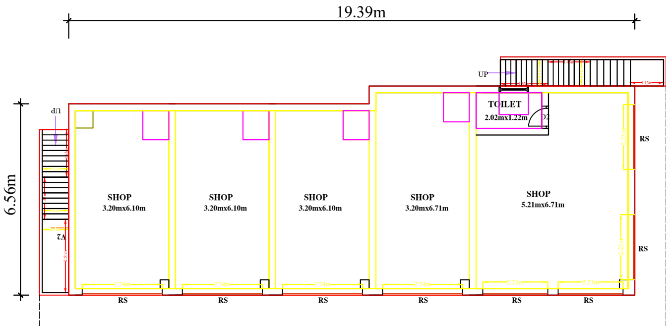
EXISTING GROUND FLOOR PLAN APPROVAL AUTHORITY
