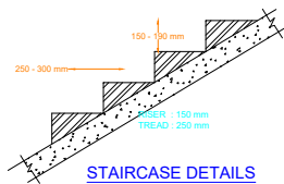
STAIRCASE DETAILS NOT TO SCALE
