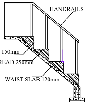
STAIRCASE DETAILS
