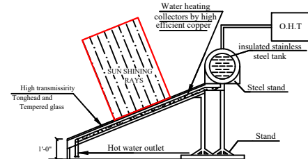
SECTION SOLAR WATER HEATER
