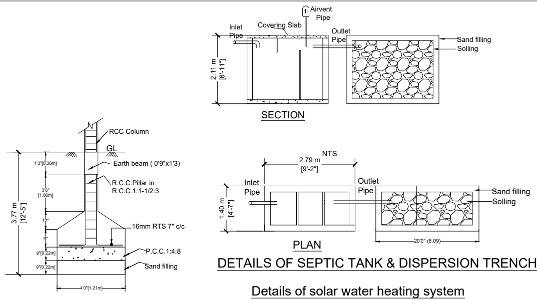
DETAILS OF SEPTIC TANK & DISPERSION TRENCH
