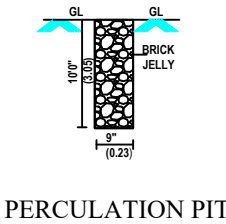
PERCOLATION PIT
