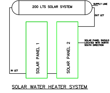
SOLAR WATER HEATER SYSTEM
