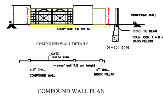
COMPOUND WALL PLAN
