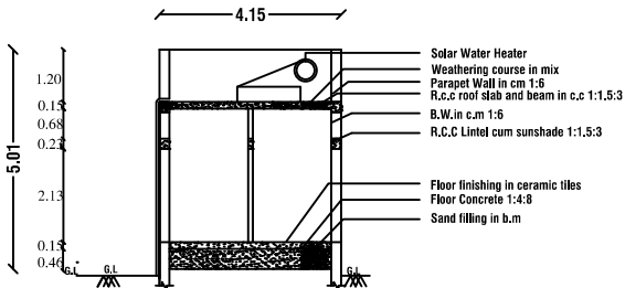
SECTION - "AB "
