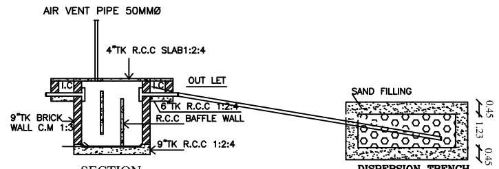
SECTION
