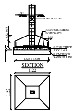
FOUNDATION DETAILS
