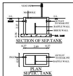
PLAN SEPTIC TANK
