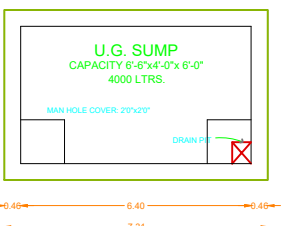
SUMP DETAIL
